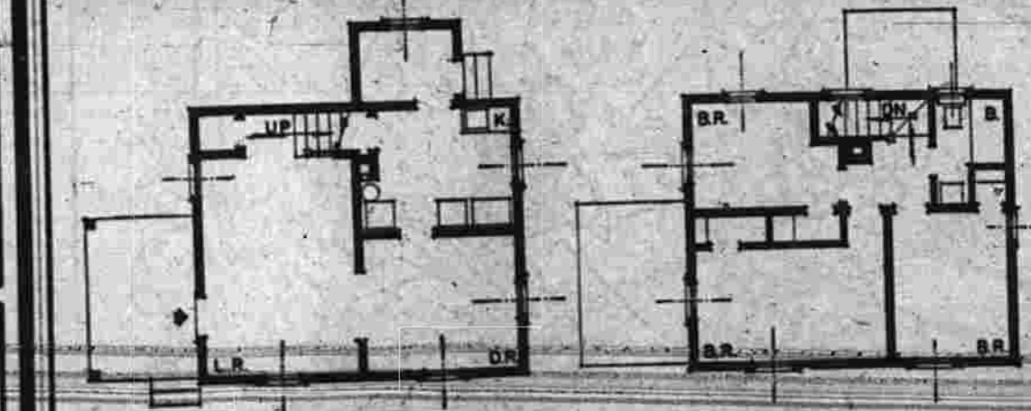
First Floor Plan Second Floor Plan
